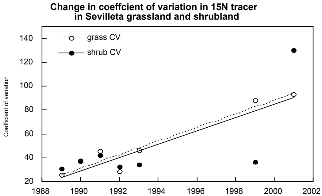
Figure 15. Coefficient of variation (CV) in the stable isotope tracer 15 N over an eleven-year period.
