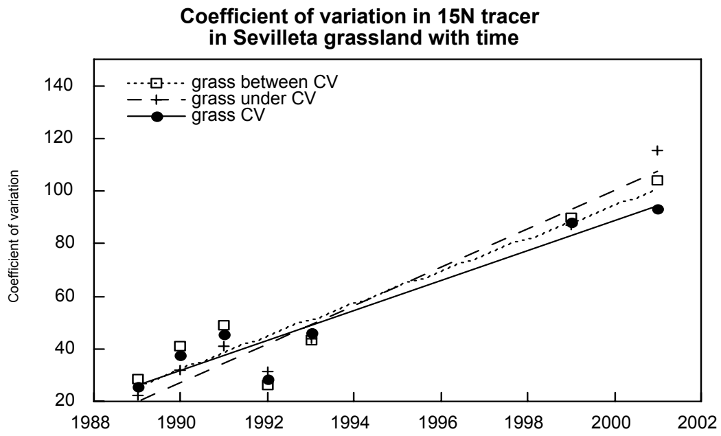
Figure. 16. Changes in the coefficient of variation (CV) in the stable isotope tracer, 15 N, under and beneath grass plants at the Sevilleta NWR.
